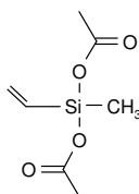
Methyl-vinyl-diacetoxysilane CAS: [2944-70-9]
