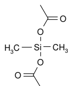
Dimethyl-diacetoxysilane CAS: [2182-66-3]
