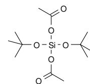
BDACDibutoxy diacetoxysilane CAS: [13170-23-5]
