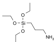
AMEO 3-Aminopropyltriethoxysilane CAS: [919-30-2]
