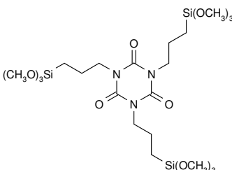
1,3,5-Tris(trimethoxysilylpropyl)-isocyanurate CAS: [26115-70-8]
