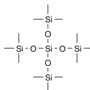
Tetrakis(trimethylsilyloxy)silane CAS: [3555-47-3]
