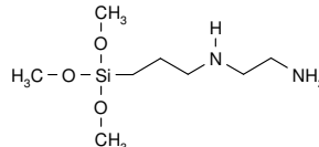
DAMO Aminoethylaminopropyltrimethoxysilane CAS: [1760-24-3]
