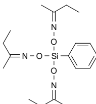
Phenyl tris (methyl ethyl ketoxime) silane CAS: [34036-80-1]
