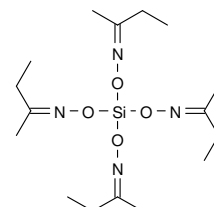
TOS Tetrakis-butanonoximsilan (40% in Toluol) CAS: [34206-40-1]
