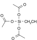
ETA-Ethyltriacetoxysilane CAS: [17689-77-9]
