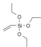
VTES Vinyltriethoxy silane CAS: [78-08-0]
