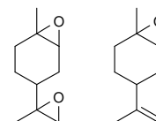
Limonene Monoxide/Limonene Dioxide (ratio 70/30) CAS: [1195-92-2]; [96-08-2]
