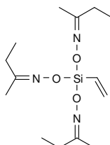
Vinox-Vinyl tris (methyl ethyl ketoxime)silane CAS: [2224-33-1]
