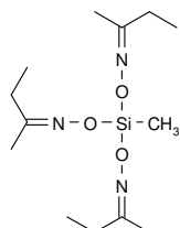
Wasox-Methyl tris (methyl ethyl ketoxime) silane CAS: [22984-54-9]
