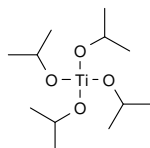
Titanium(IV) isopropoxide CAS: [546-68-9]
