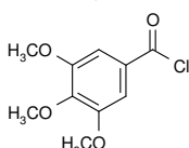
3,4,5-Trimethoxybenzoyl Chloride CAS: [4521-61-3]
