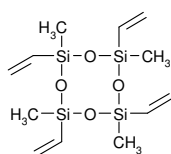
Tetramethyl-tetravinyl-cyclotetra-siloxane CAS: [2554-06-5]
