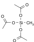
MTA-Methyltriacetoxysilane CAS: [4253-34-3]
