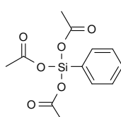
Phenyltriacetoxysilane CAS: [18042-54-1]
