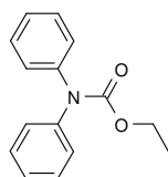
Diphenyl Urethane (DPU) CAS: [603-52-1]
