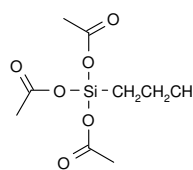
PTA-Propyltriacetoxysilane CAS: [17865-07-5]
